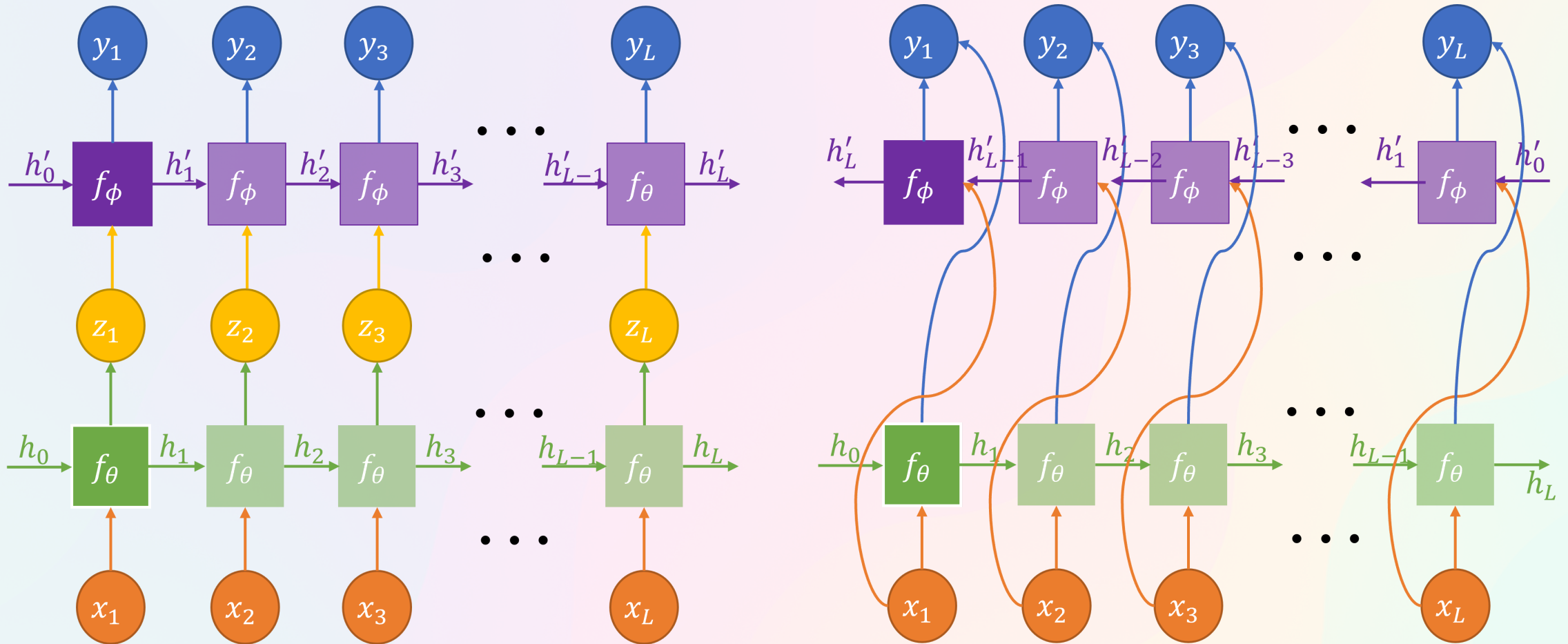
Bidirectional RNN
